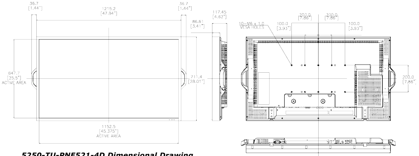
5250-TU-PNE521-4D Dimensional Drawing
