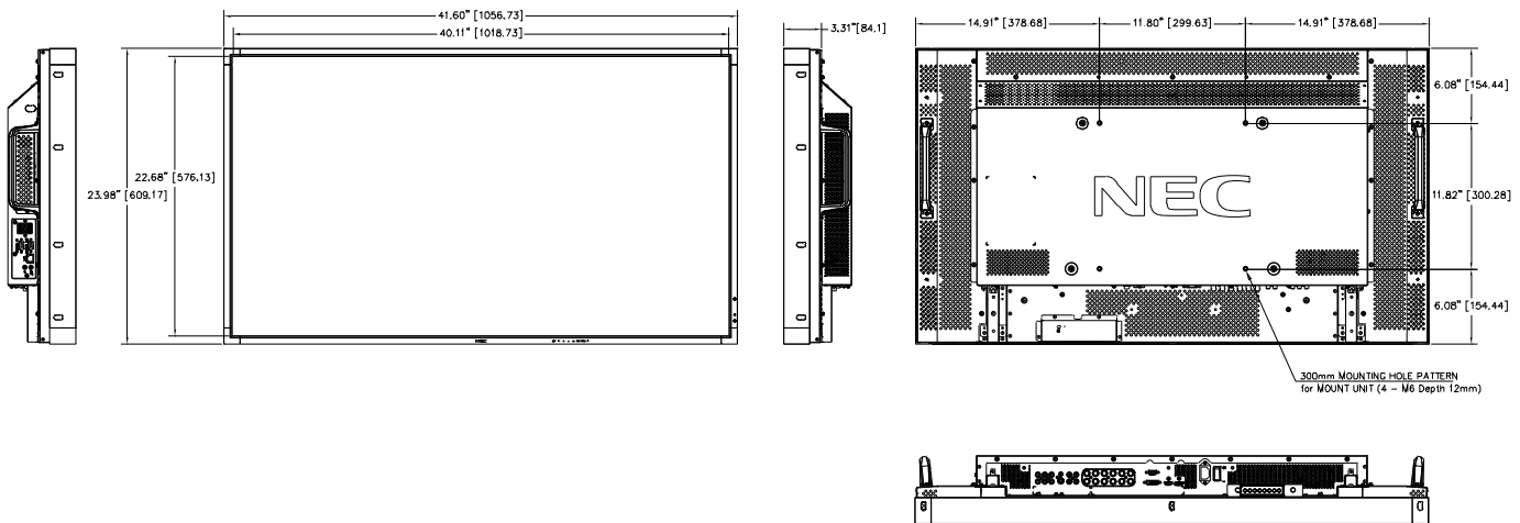
NEC P461 Dimensional Drawing
