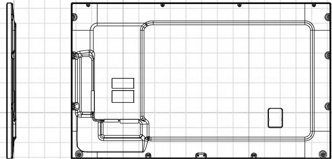
4050EX, 4050EXn Samsung Dimensional Drawing
