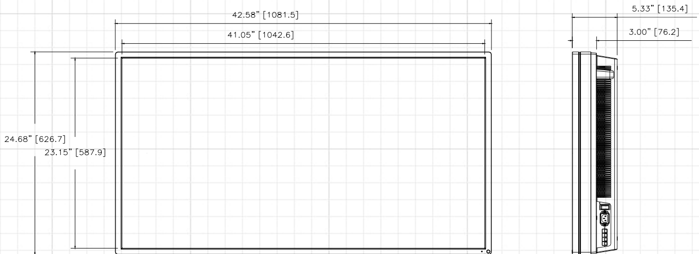
4750 Sony Dimensional Drawing
